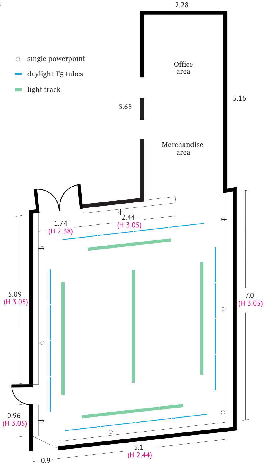
Run Amok floor plan
